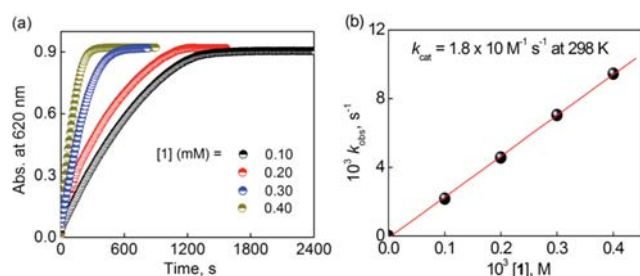
Figure 3. (a) Time profiles of the absorbance at 620 nm due to \text{Fc}^+ in the two-electron reduction of \text{O}_2 ( [\text{O}_2] = 1.0 mM) catalyzed by 1 (0.10 mM (black), 0.20 mM (red), 0.30 mM (blue), and 0.40 mM (dark yellow)) with \text{Fc} (10 mM) in the presence of \text{HClO}_4 (60 mM) in acetone solution at 298 K. (b) Plot of k_{\text{obs}} versus [\text{I}] for the two-electron reduction of \text{O}_2 ( [\text{O}_2] = 1.0 mM) catalyzed by 1 with \text{Fc} (10 mM) in the presence of \text{HClO}_4 (60 mM) in acetone at 298 K.
