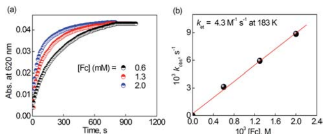
Figure 6. (a) Time profiles of the absorbance at 620 nm due to \text{Fc}^+ in the electron transfer reaction from \text{Fc} (0.60 mM (black), 1.3 mM (red), and 2.0 mM (blue)) to 1 (0.10 mM) in acetone at 183 K. (b) Plot of k_{\text{obs}} versus [\text{Fc}] in the electron transfer from \text{Fc} to [\text{Cu}^{\text{II}}(\text{tepa})]^{2+} ( 1 ; 0.10 mM) in acetone solution at 183 K.
